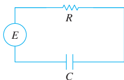
FIGURE 3.1.8 RC-series circuit
